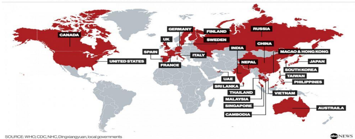
Fig 1 Countries with confirmed Corona Virus Cases 2
